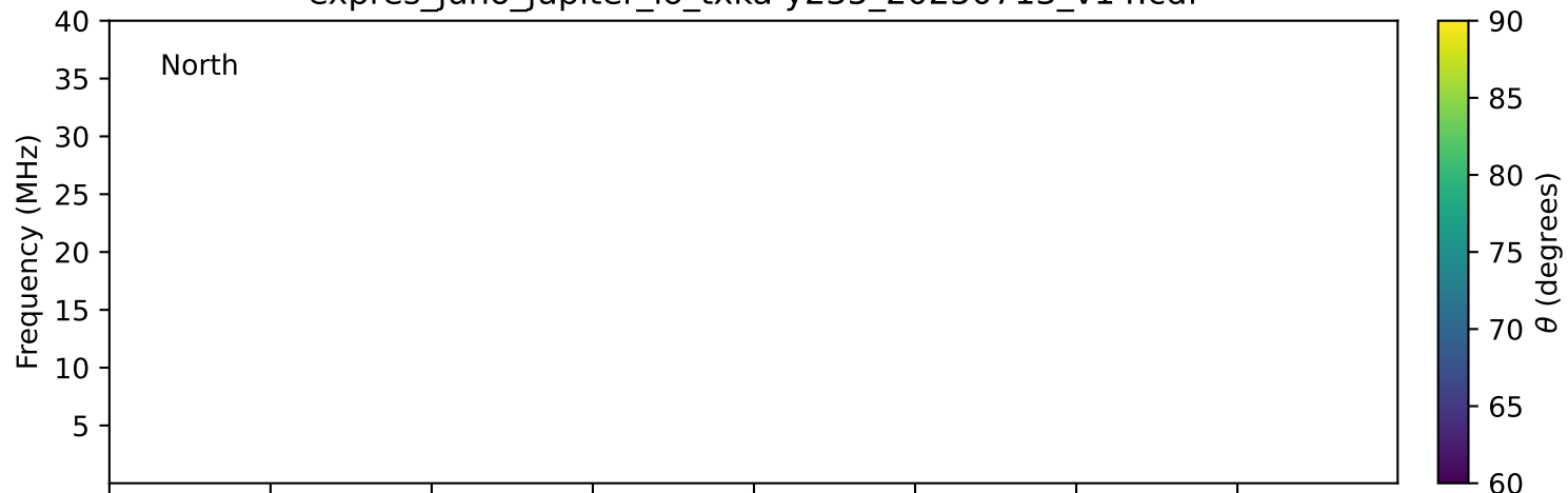
expres_juno_jupiter_io_txka-y235_20250713_v14.cdf
