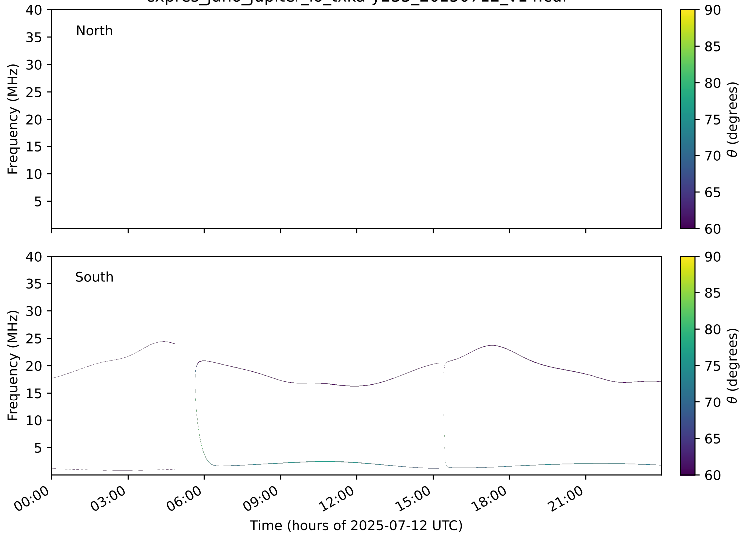
expres_juno_jupiter_io_txka-y235_20250712_v14.cdf
