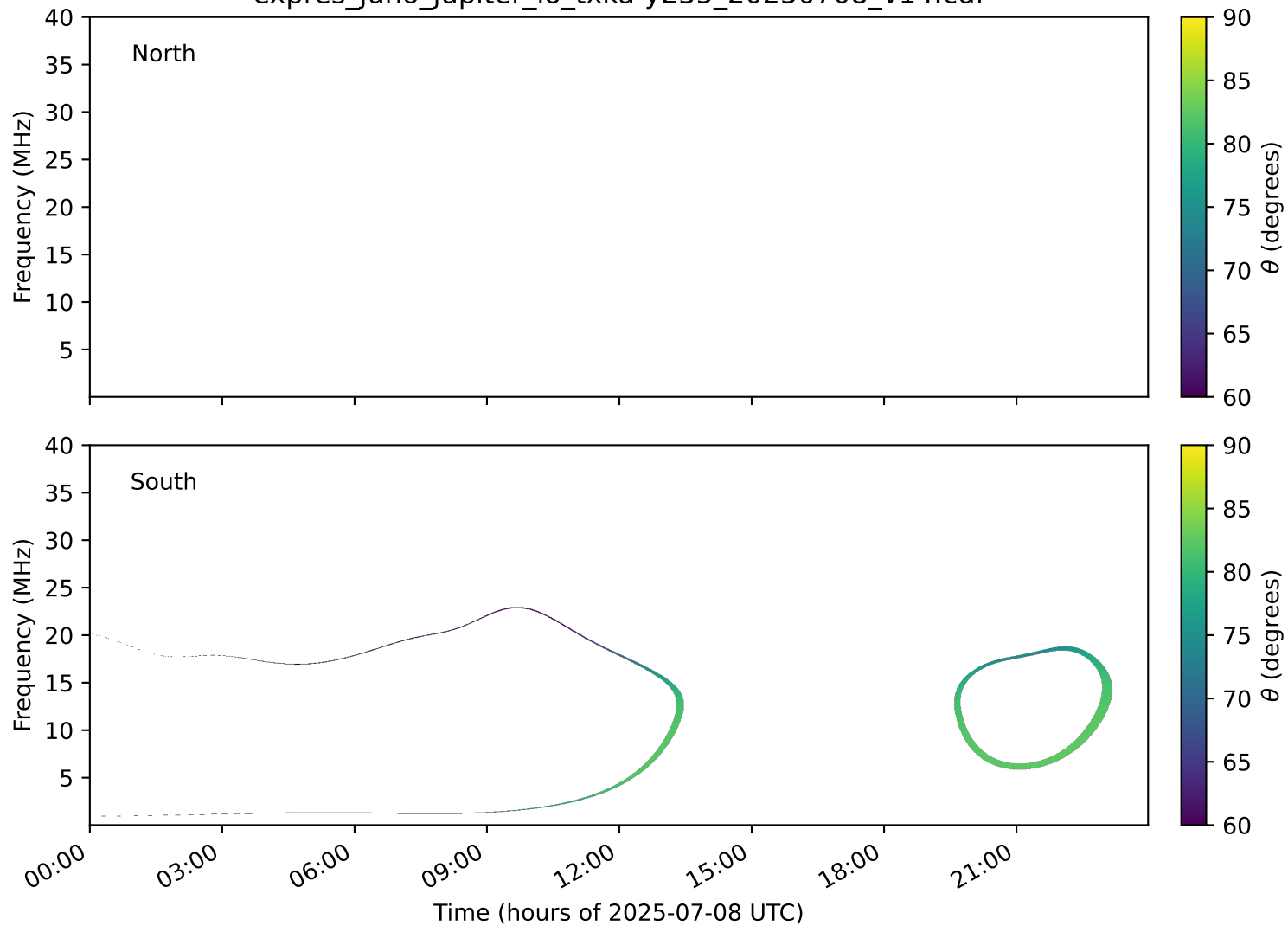
expres_juno_jupiter_io_txka-y235_20250708_v14.cdf
