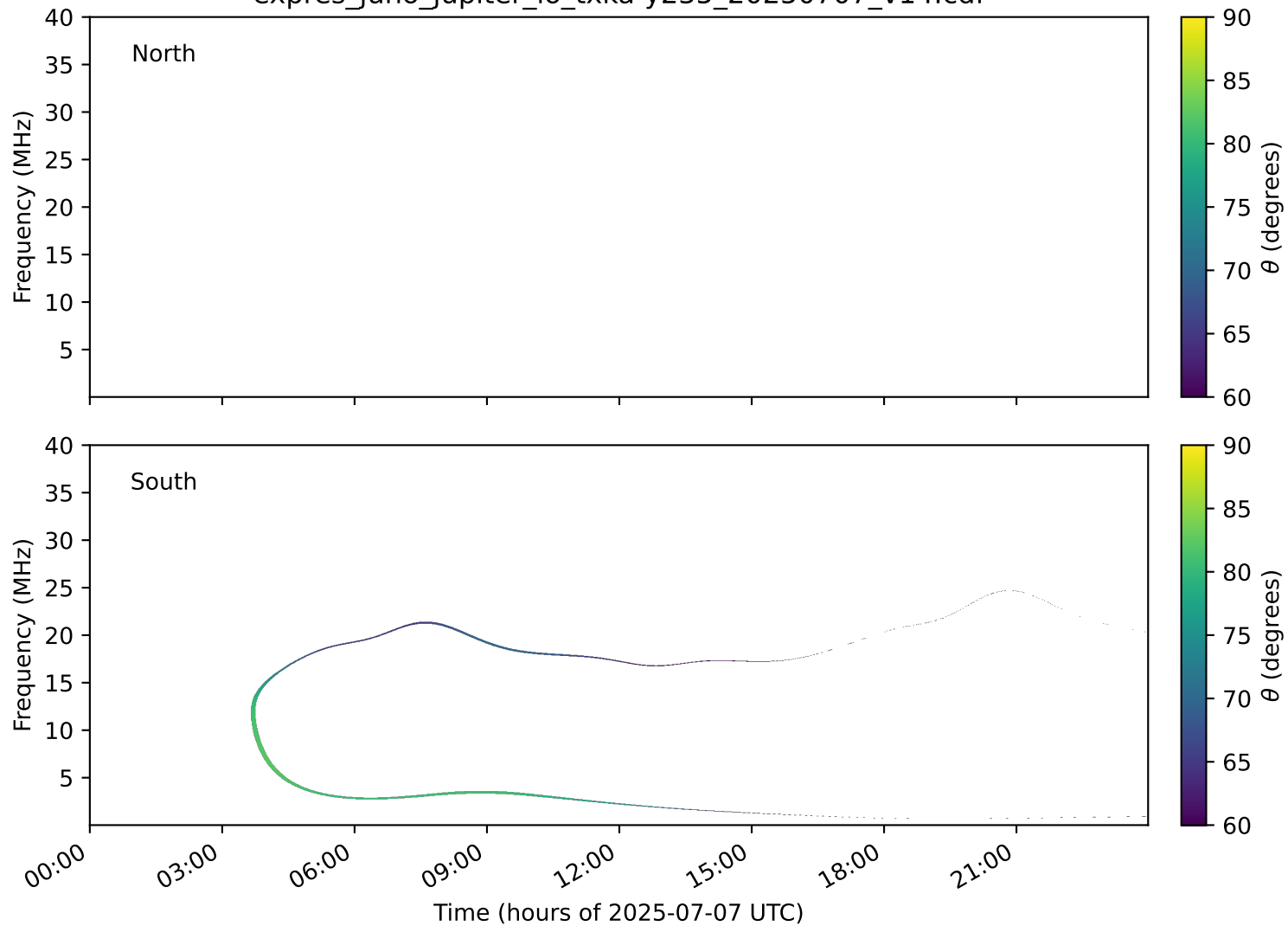
expres_juno_jupiter_io_txka-y235_20250707_v14.cdf
