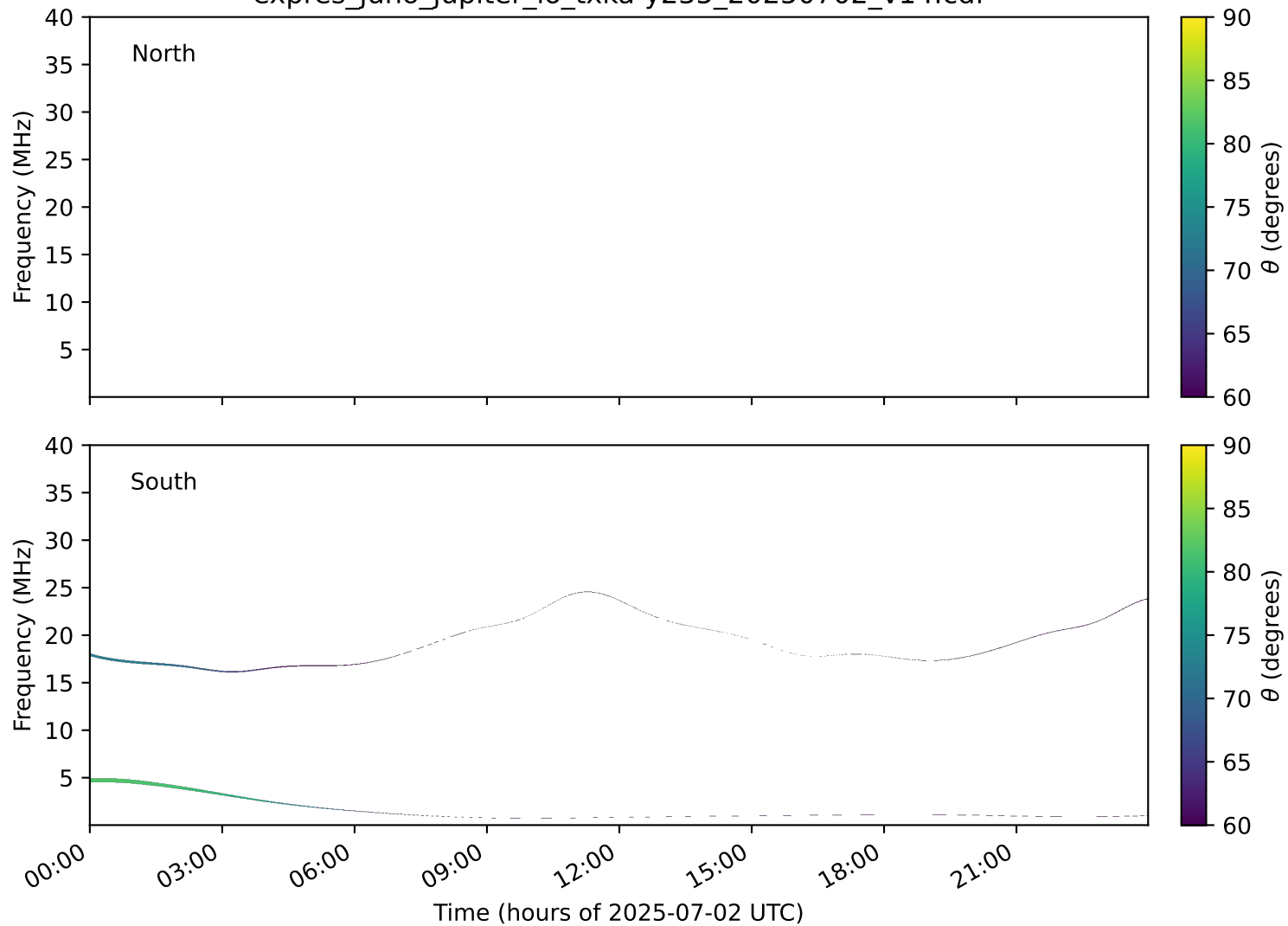
expres_juno_jupiter_io_txka-y235_20250702_v14.cdf
