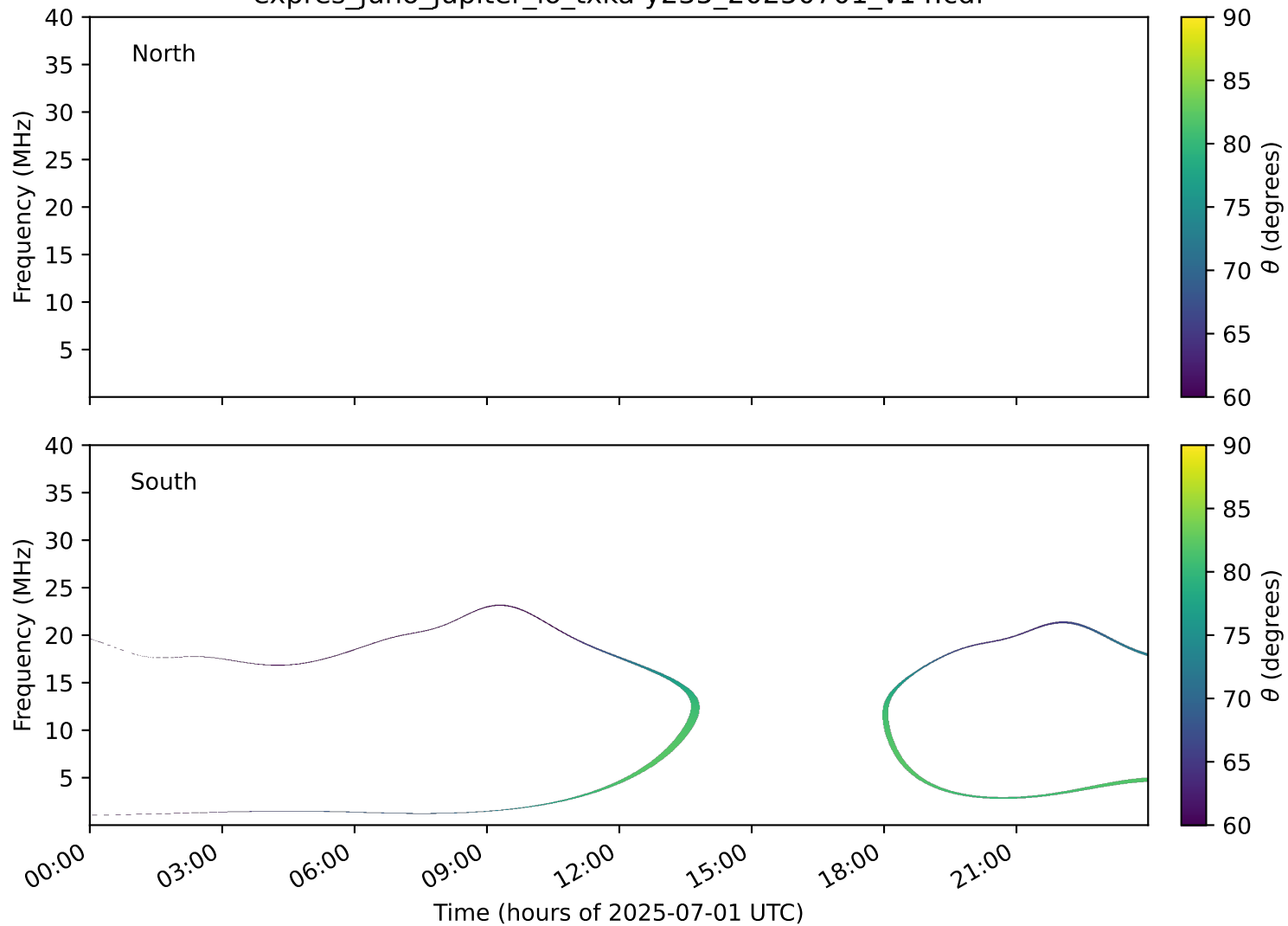
expres_juno_jupiter_io_txka-y235_20250701_v14.cdf
