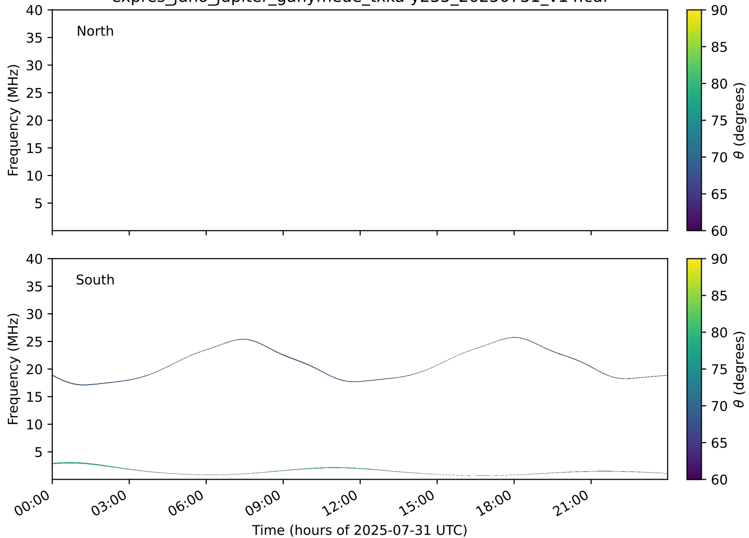
expres_juno_jupiter_ganymede_txka-y235_20250731_v14.cdf
