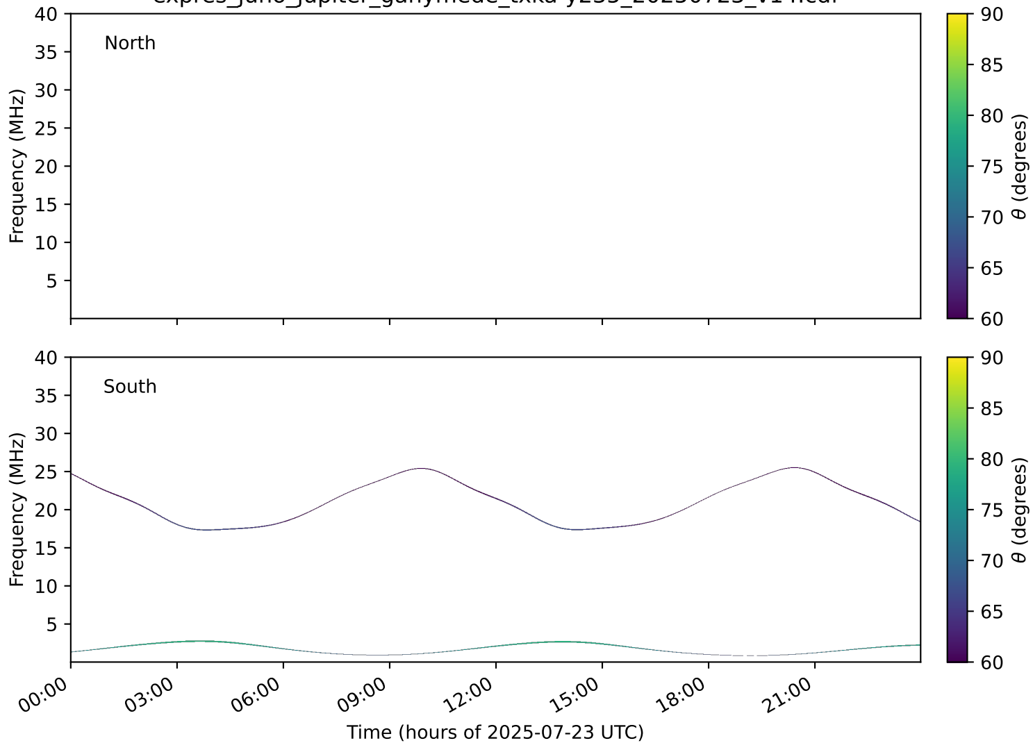
expres_juno_jupiter_ganymede_txka-y235_20250723_v14.cdf
