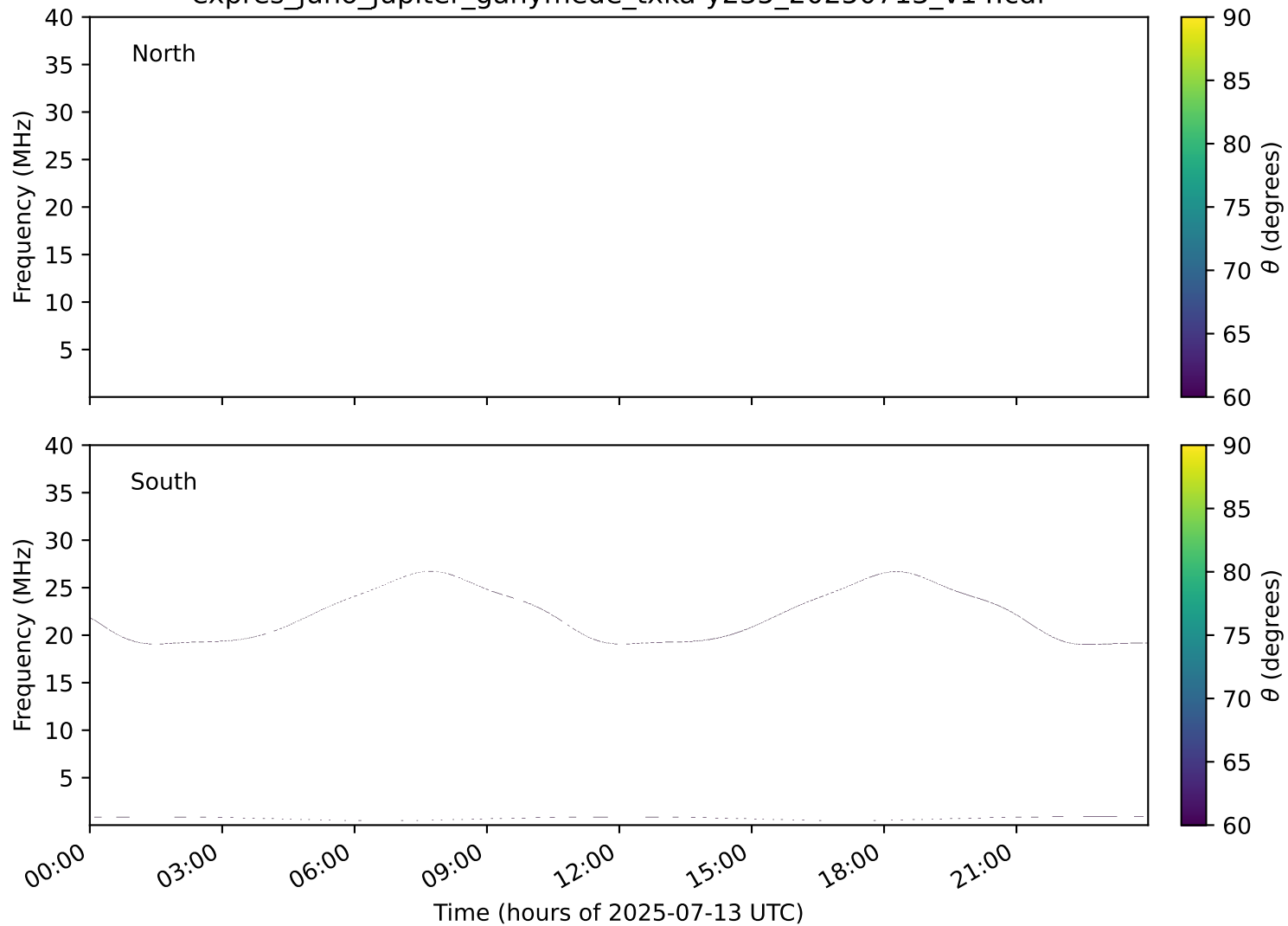
expres_juno_jupiter_ganymede_txka-y235_20250713_v14.cdf
