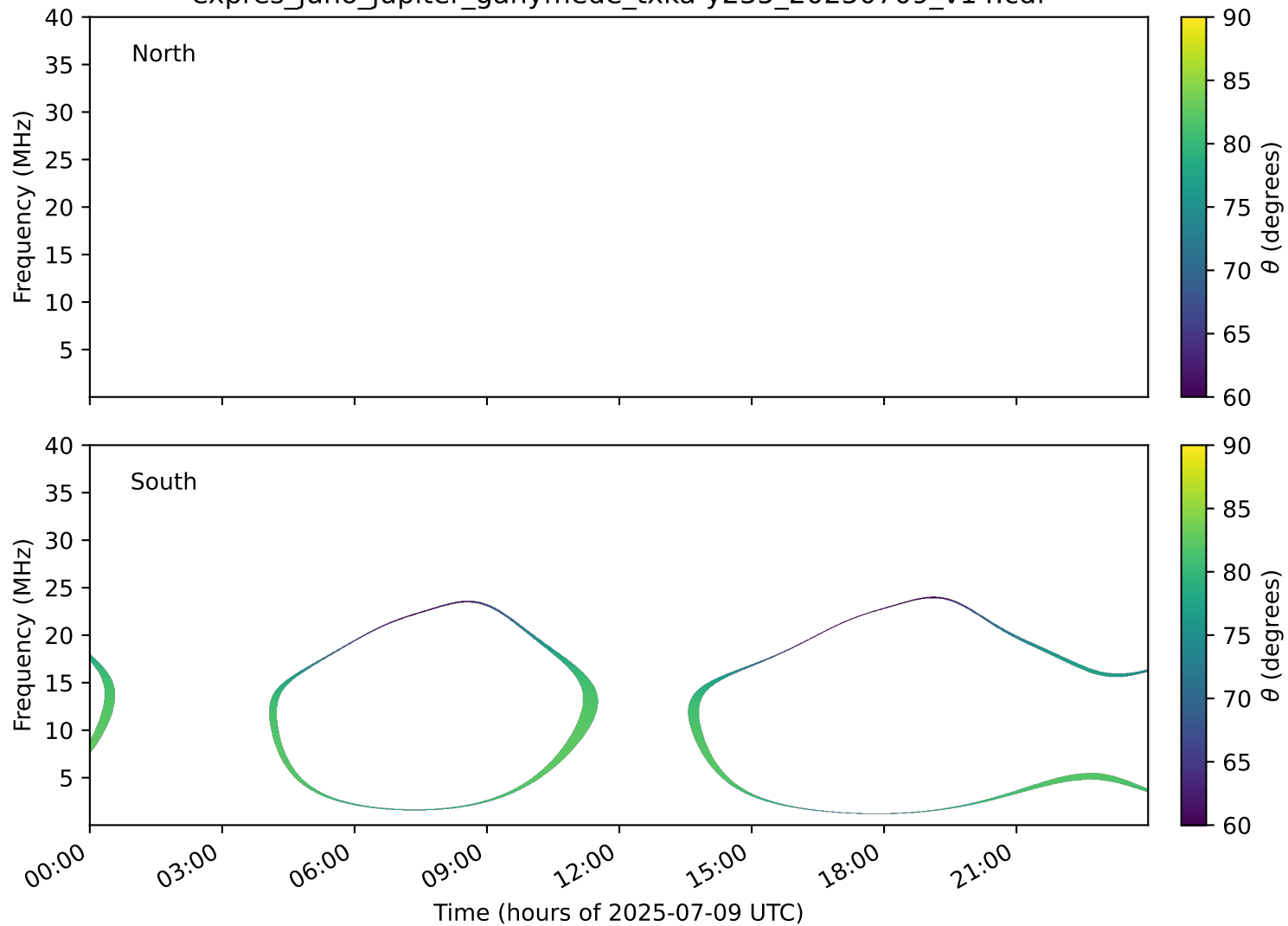
expres_juno_jupiter_ganymede_txka-y235_20250709_v14.cdf
