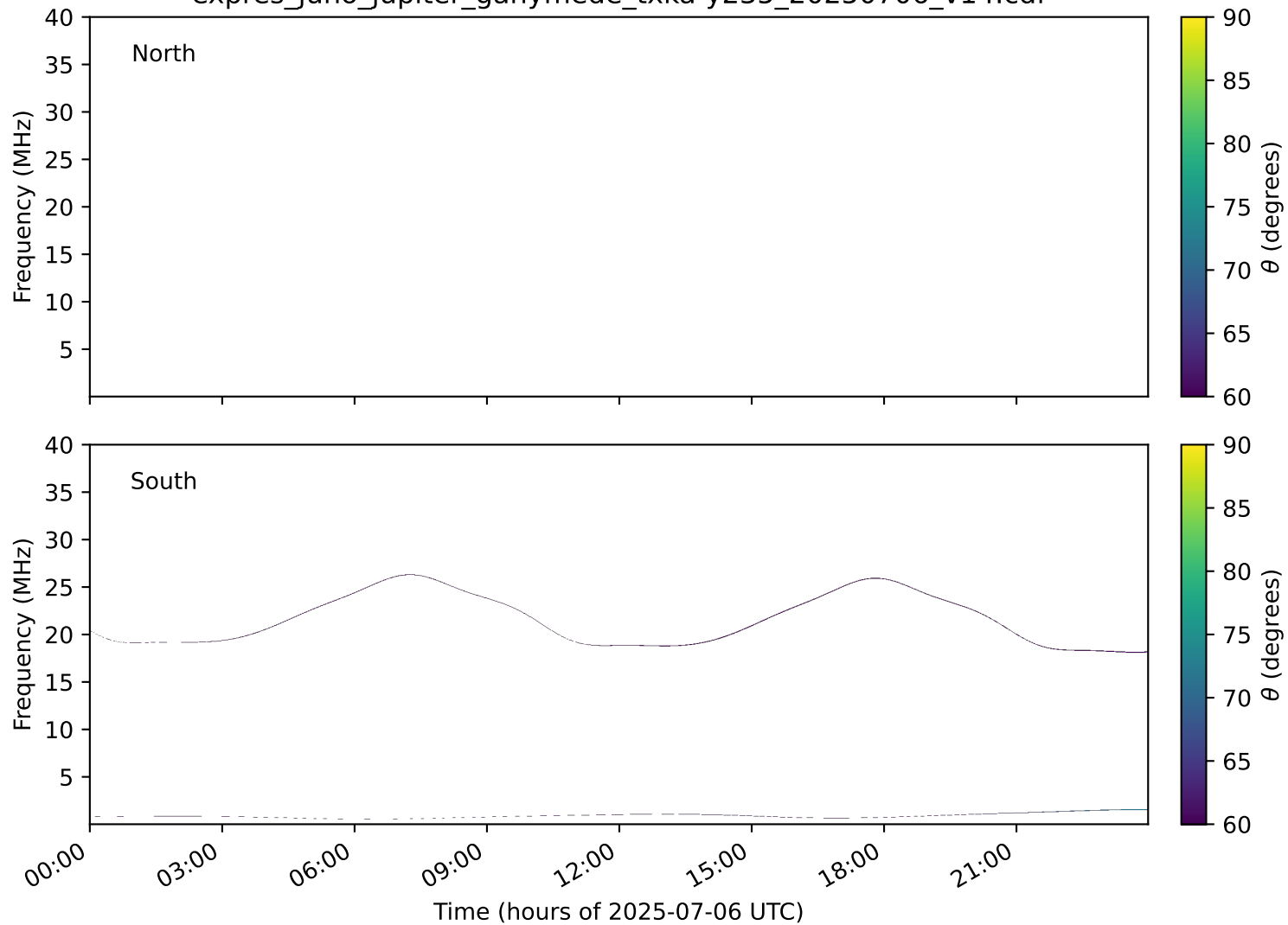
expres_juno_jupiter_ganymede_txka-y235_20250706_v14.cdf
