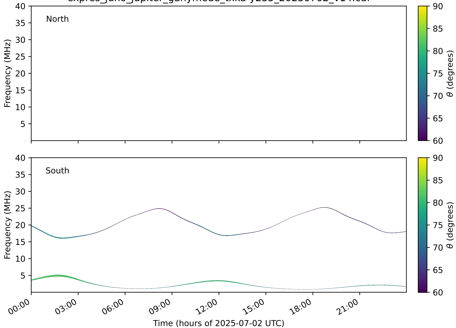
expres_juno_jupiter_ganymede_txka-y235_20250702_v14.cdf
