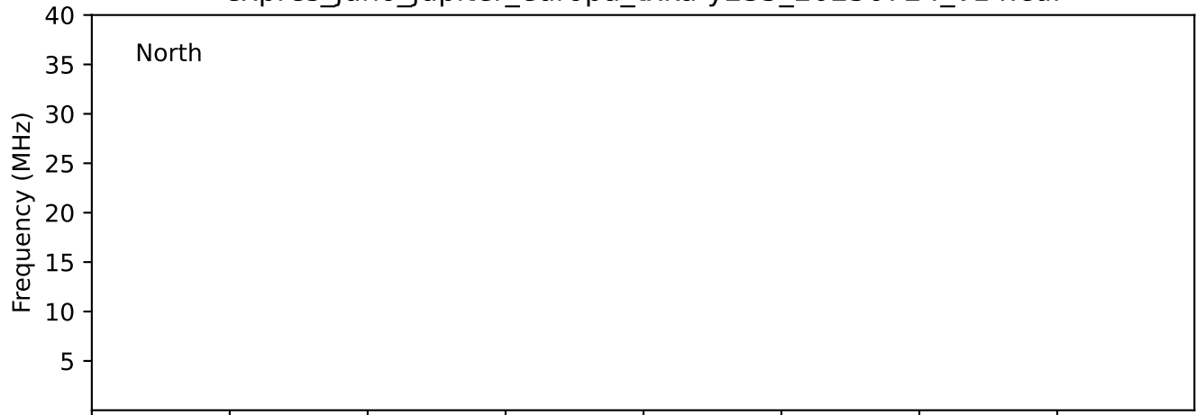
expres_juno_jupiter_europa_txka-y235_20250724_v14.cdf
