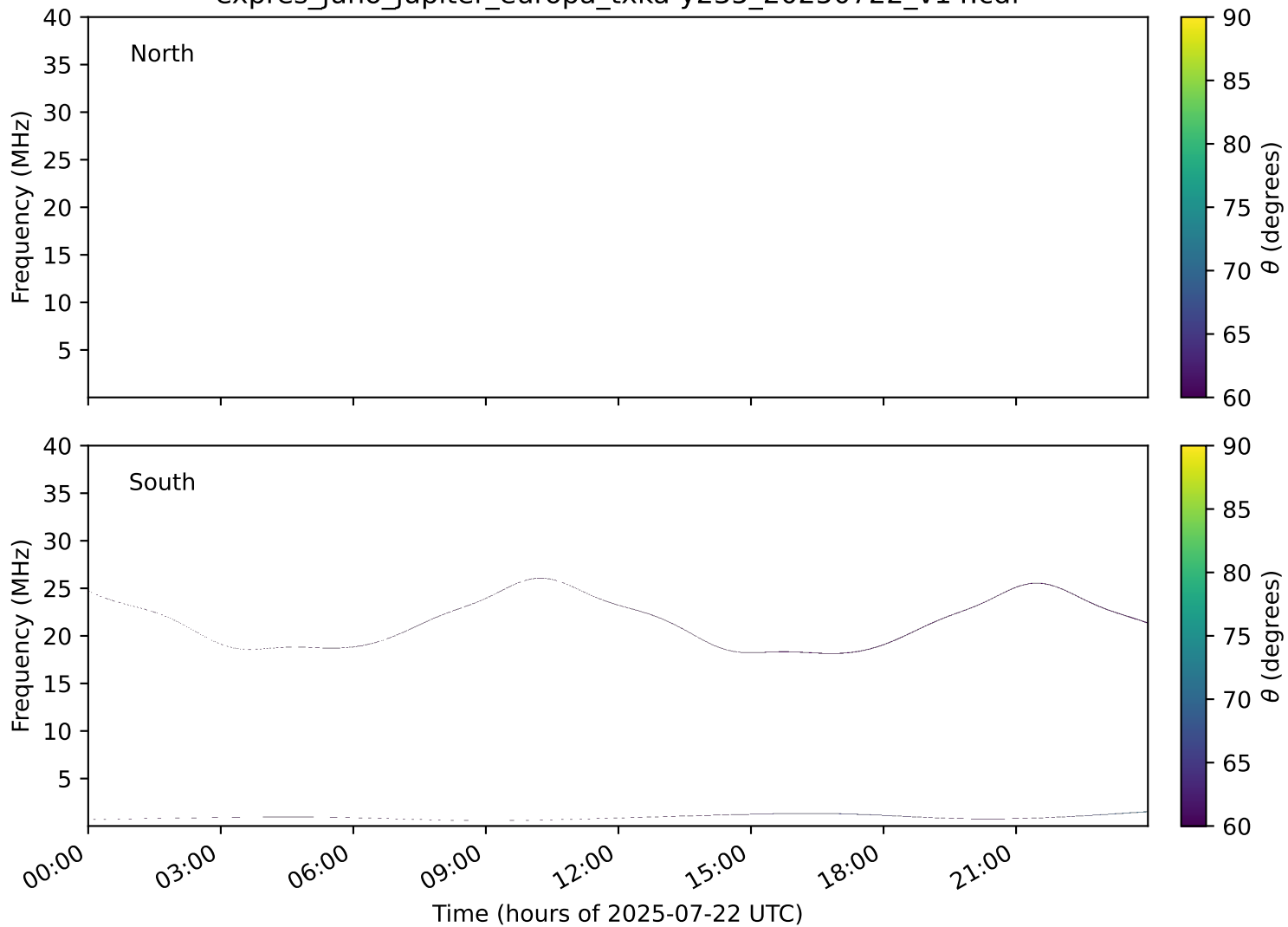
expres_juno_jupiter_europa_txka-y235_20250722_v14.cdf
