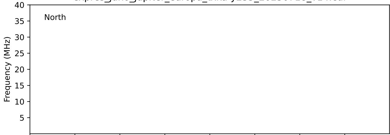
expres_juno_jupiter_europa_txka-y235_20250718_v14.cdf
