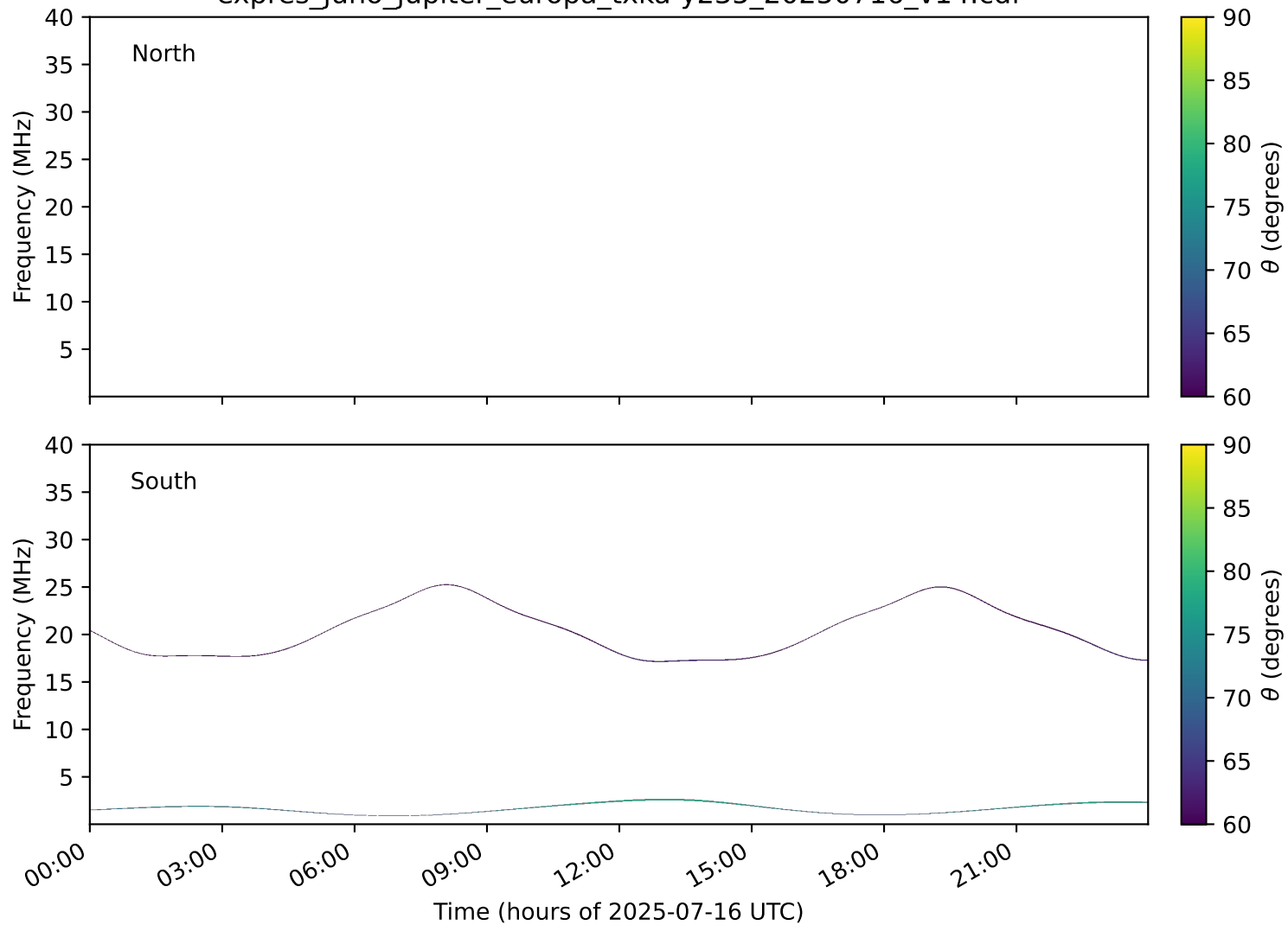
expres_juno_jupiter_europa_txka-y235_20250716_v14.cdf
