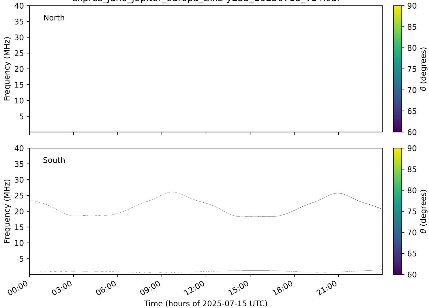
expres_juno_jupiter_europa_txka-y235_20250715_v14.cdf
