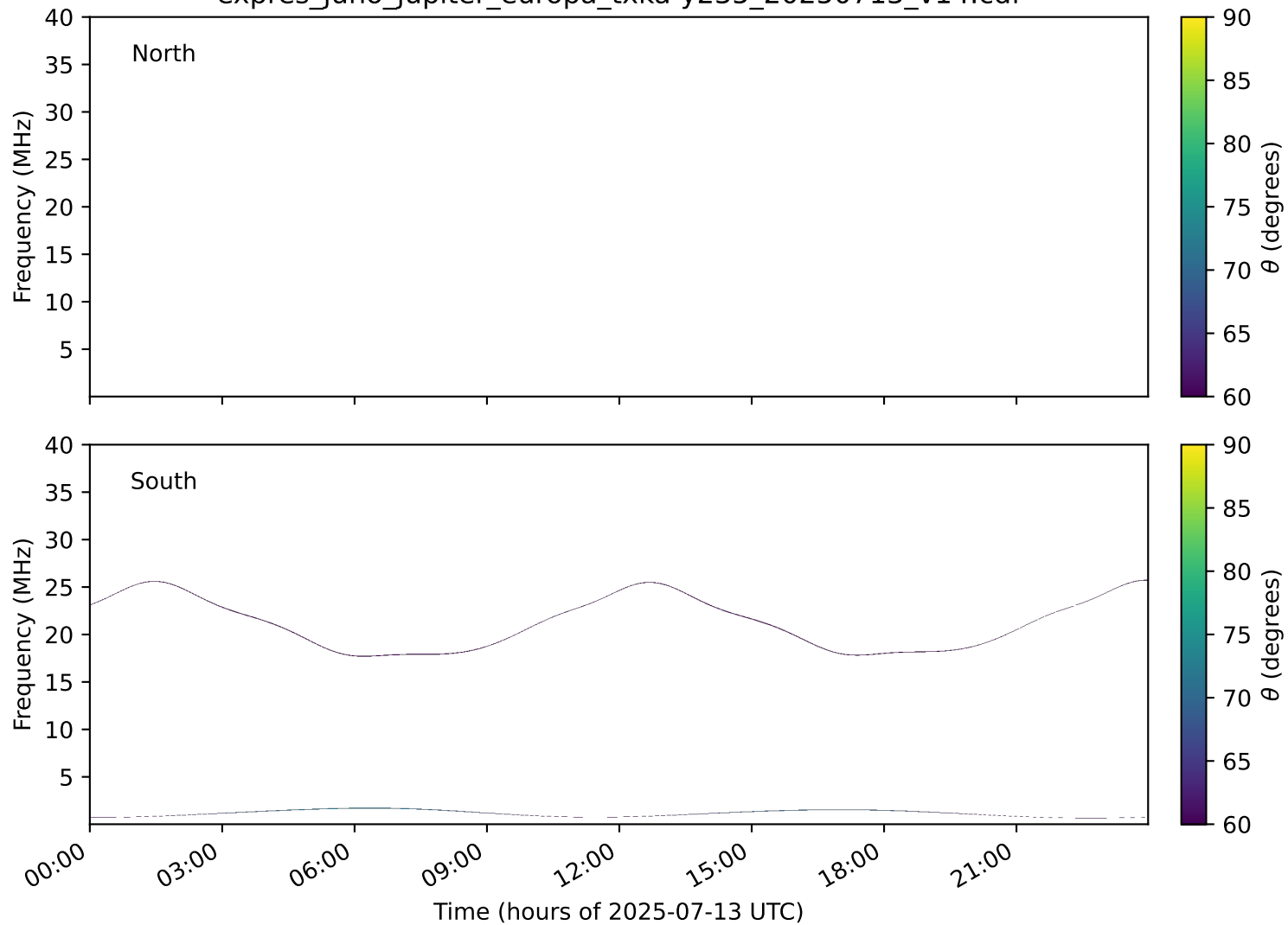
expres_juno_jupiter_europa_txka-y235_20250713_v14.cdf
