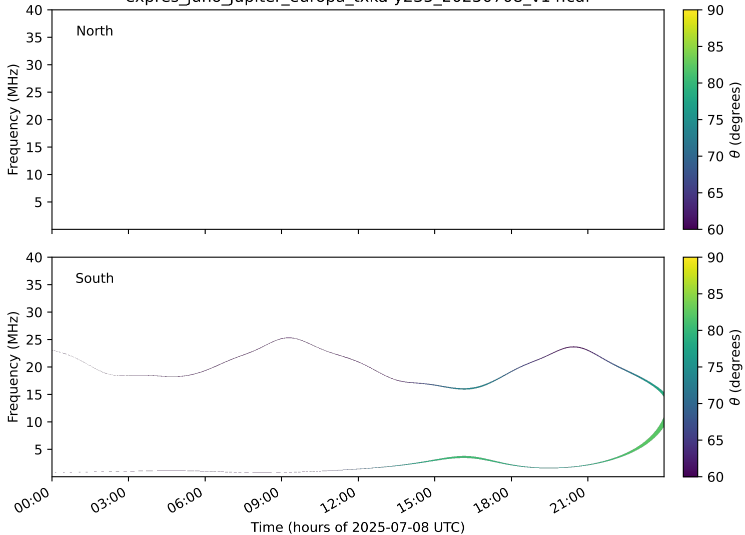
expres_juno_jupiter_europa_txka-y235_20250708_v14.cdf
