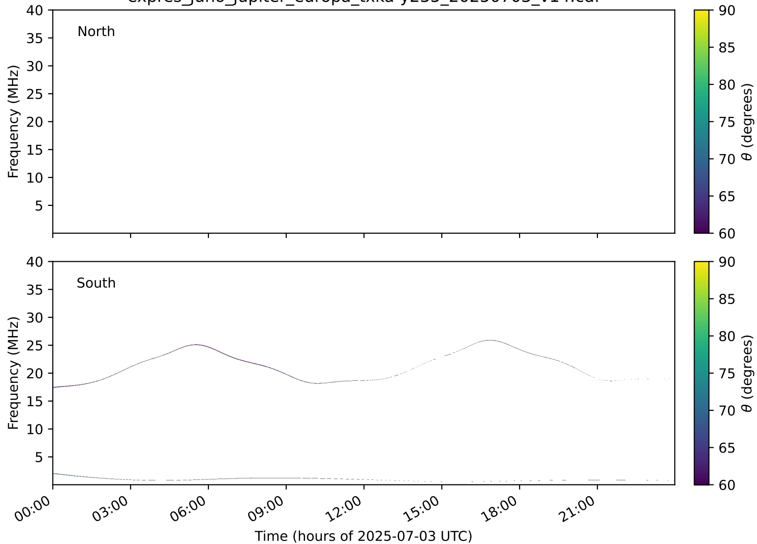
expres_juno_jupiter_europa_txka-y235_20250703_v14.cdf
