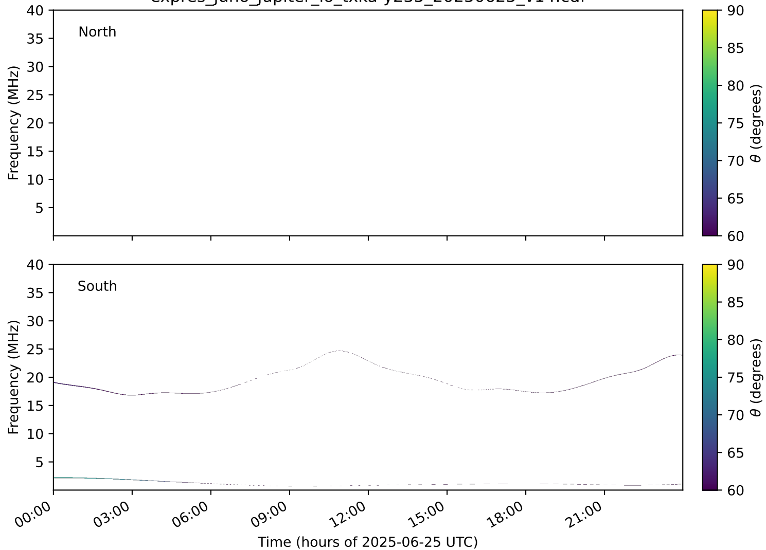
expres_juno_jupiter_io_txka-y235_20250625_v14.cdf
