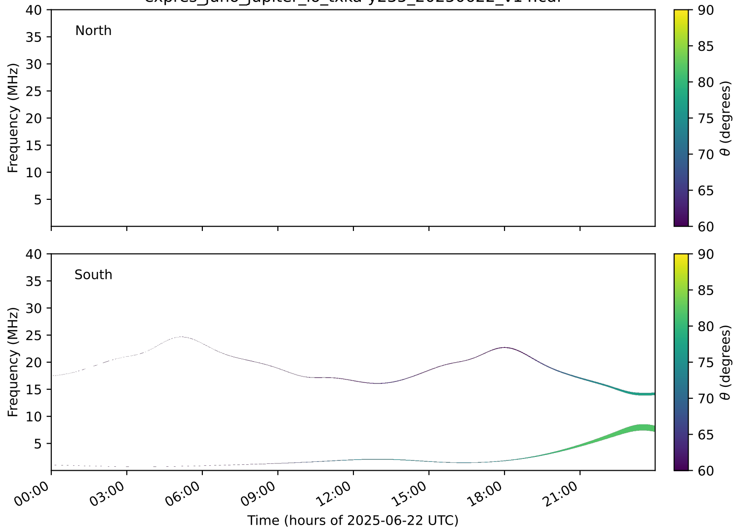
expres_juno_jupiter_io_txka-y235_20250622_v14.cdf
