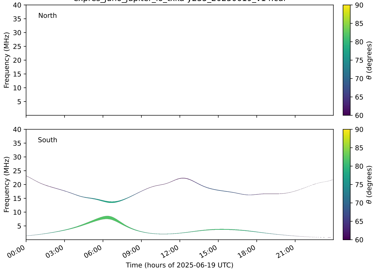
expres_juno_jupiter_io_txka-y235_20250619_v14.cdf
