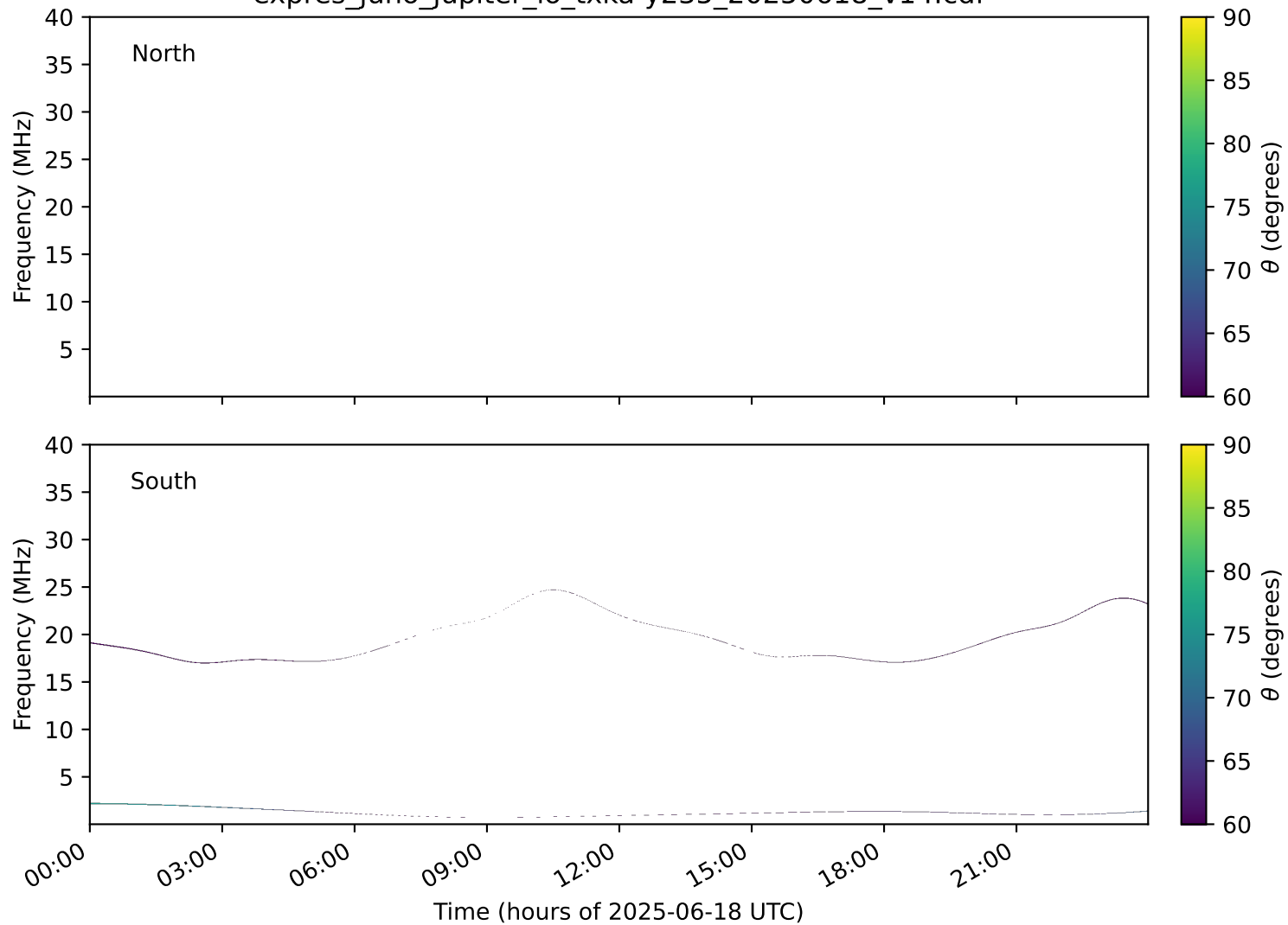
expres_juno_jupiter_io_txka-y235_20250618_v14.cdf
