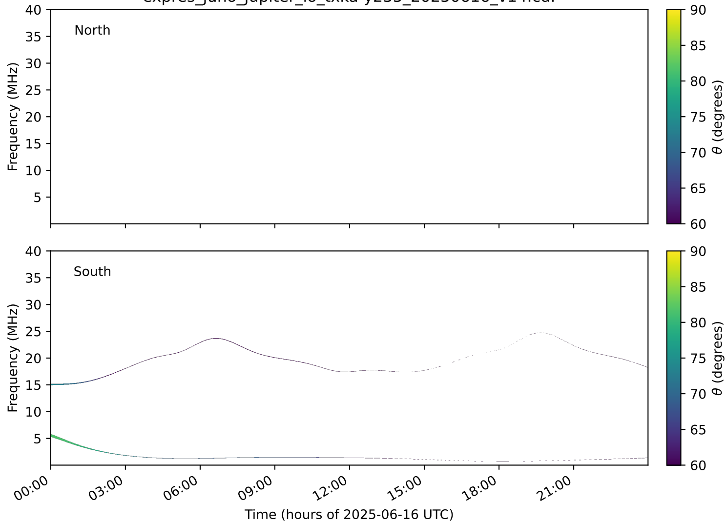
expres_juno_jupiter_io_txka-y235_20250616_v14.cdf
