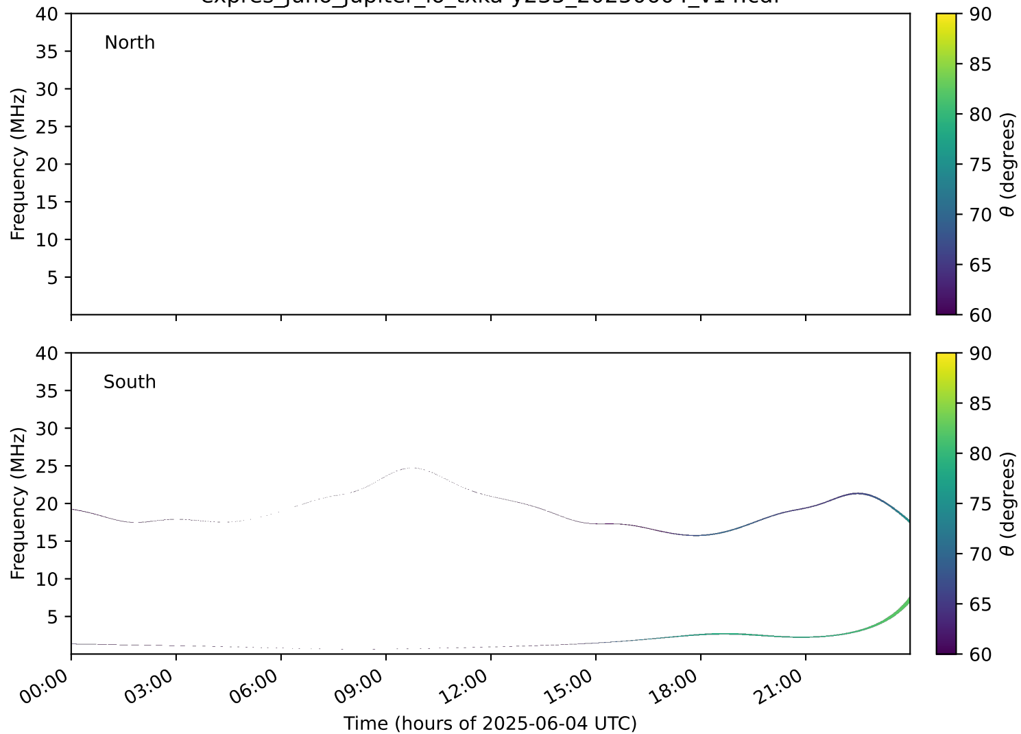
expres_juno_jupiter_io_txka-y235_20250604_v14.cdf
