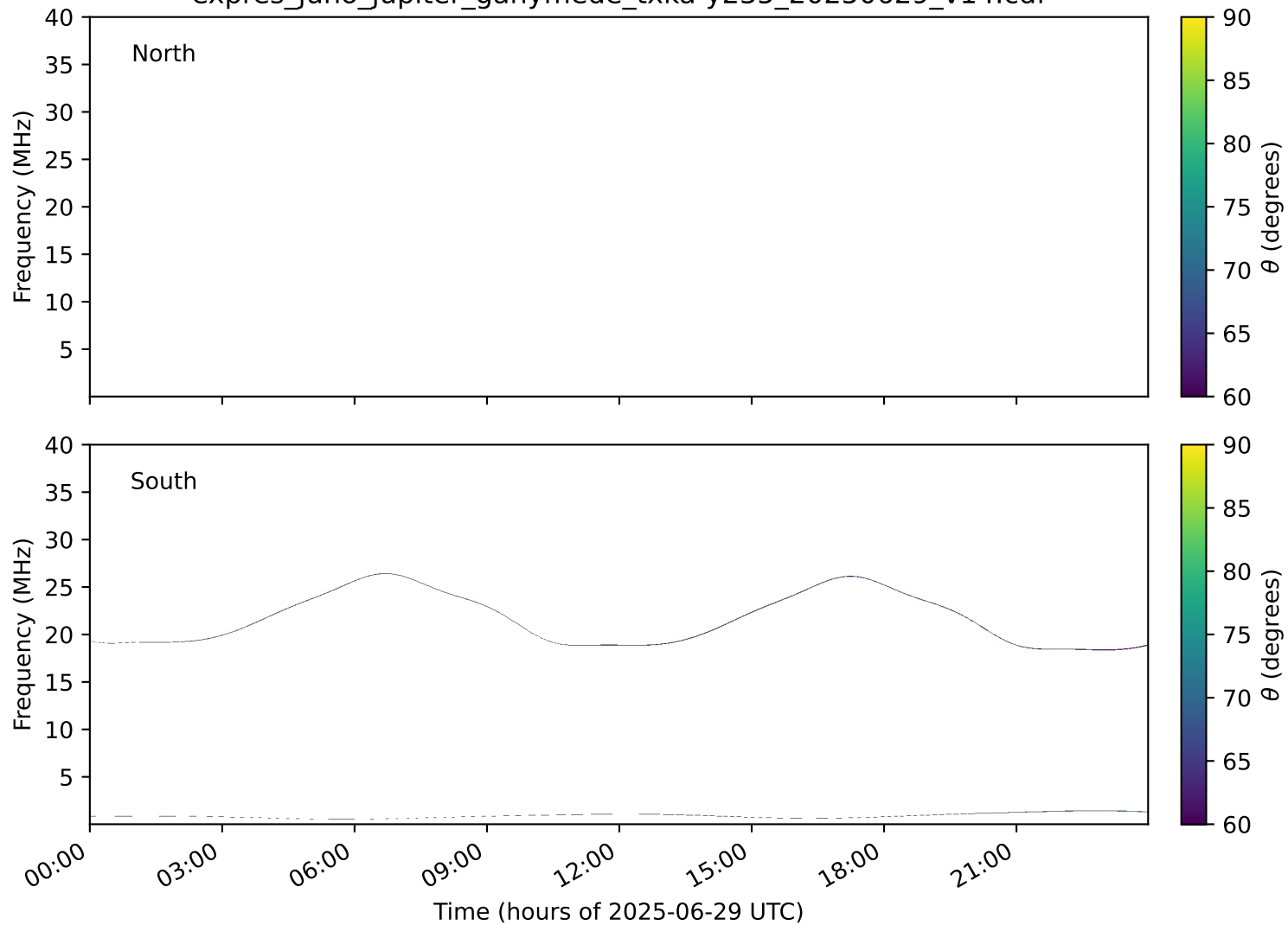
expres_juno_jupiter_ganymede_txka-y235_20250629_v14.cdf
