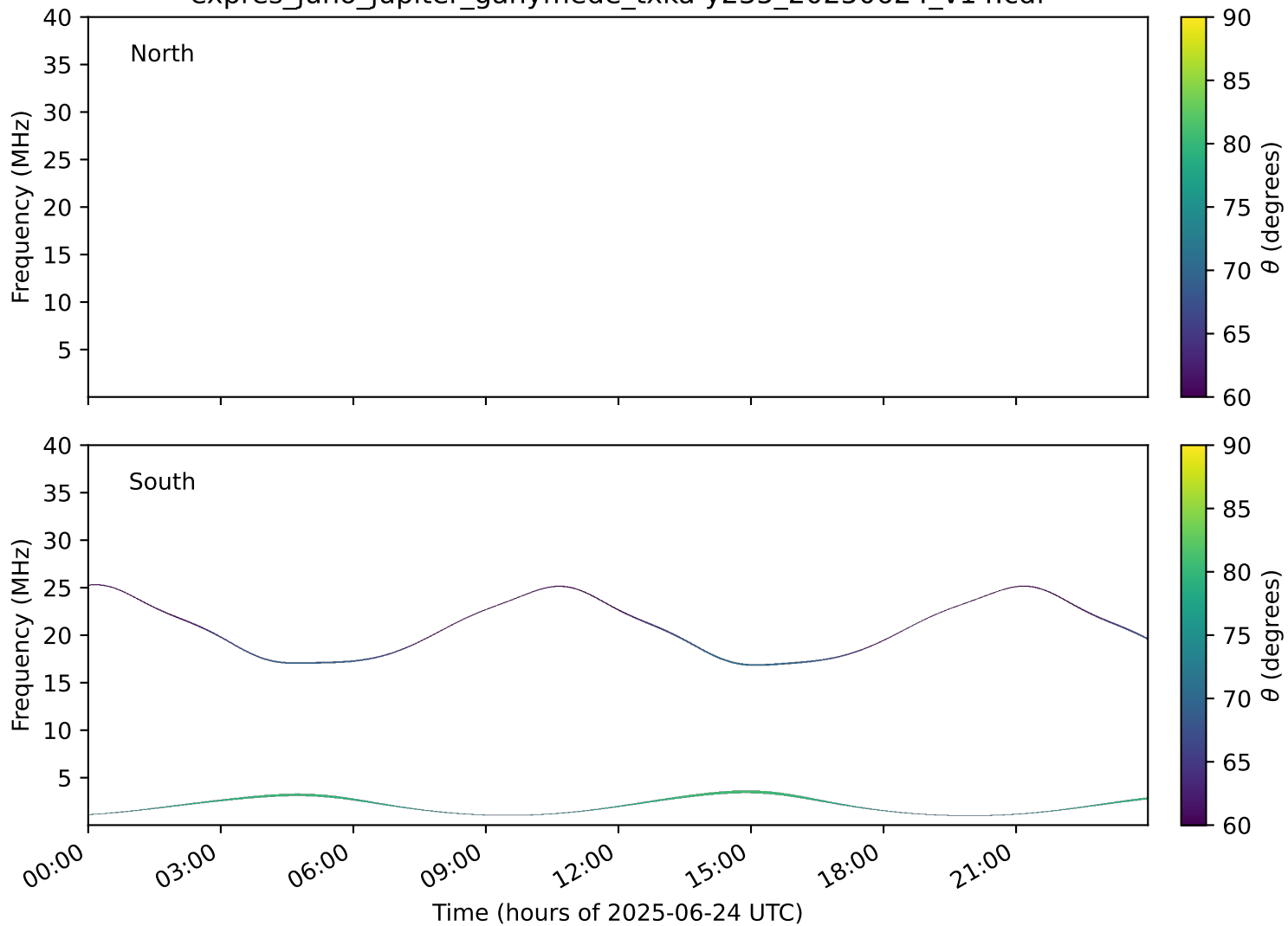
expres_juno_jupiter_ganymede_txka-y235_20250624_v14.cdf
