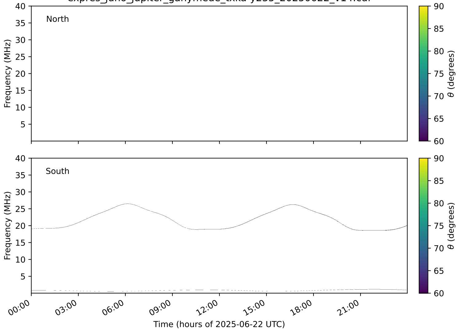
expres_juno_jupiter_ganymede_txka-y235_20250622_v14.cdf
