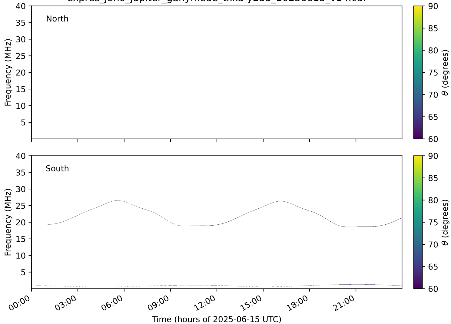
expres_juno_jupiter_ganymede_txka-y235_20250615_v14.cdf
