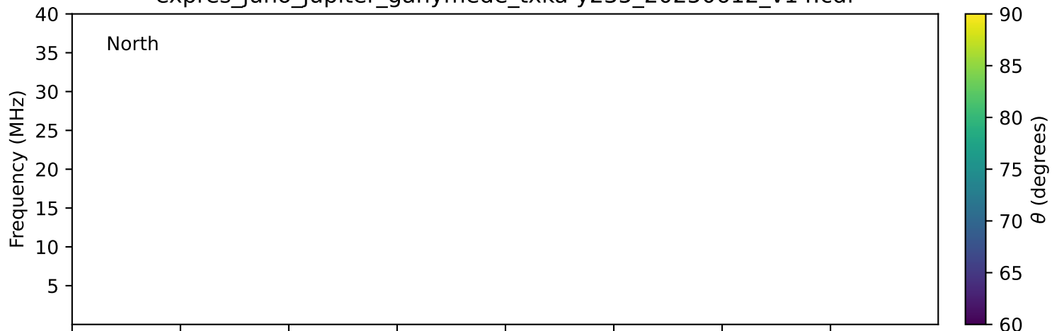
expres_juno_jupiter_ganymede_txka-y235_20250612_v14.cdf
