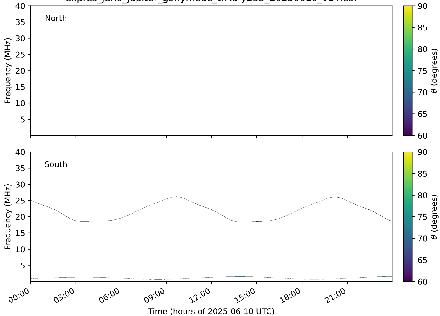
expres_juno_jupiter_ganymede_txka-y235_20250610_v14.cdf
