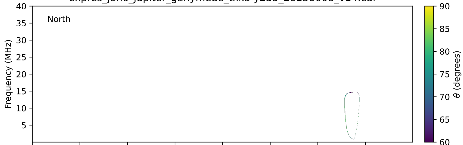
expres_juno_jupiter_ganymede_txka-y235_20250608_v14.cdf
