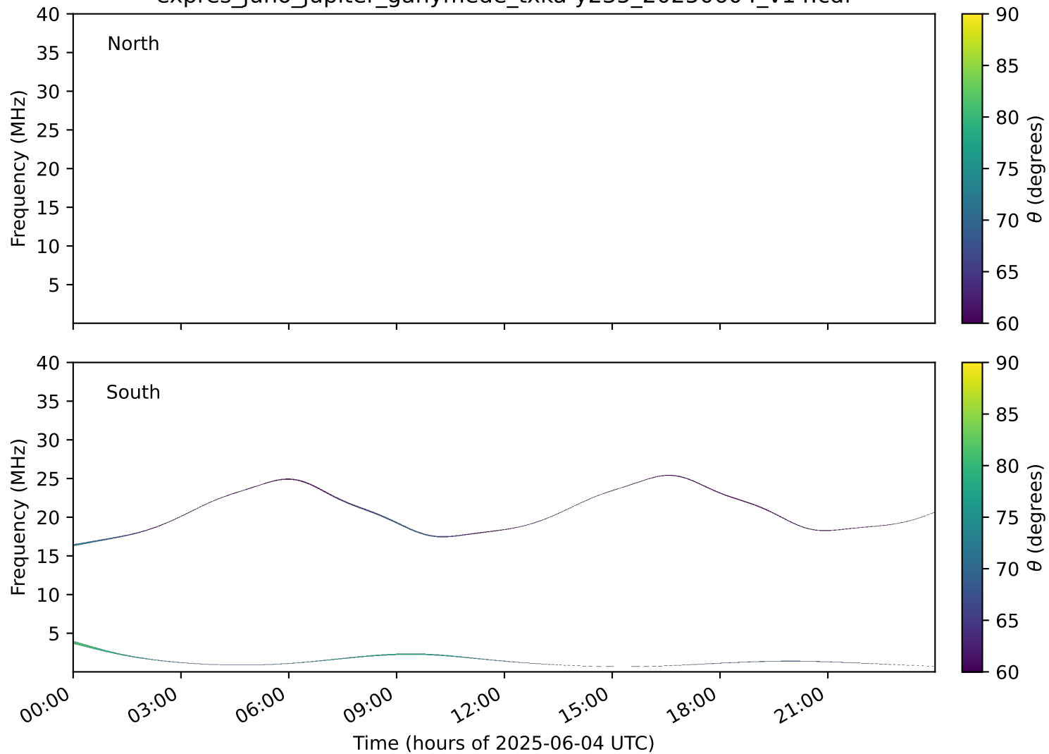
expres_juno_jupiter_ganymede_txka-y235_20250604_v14.cdf
