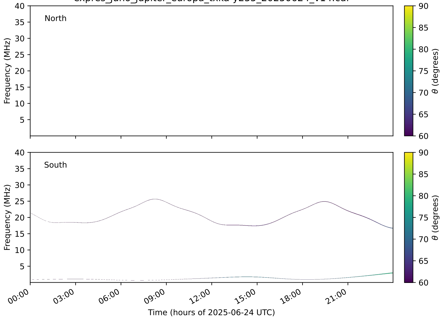
expres_juno_jupiter_europa_txka-y235_20250624_v14.cdf
