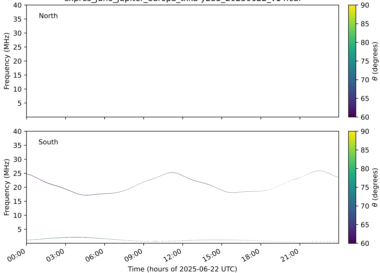
expres_juno_jupiter_europa_txka-y235_20250622_v14.cdf
