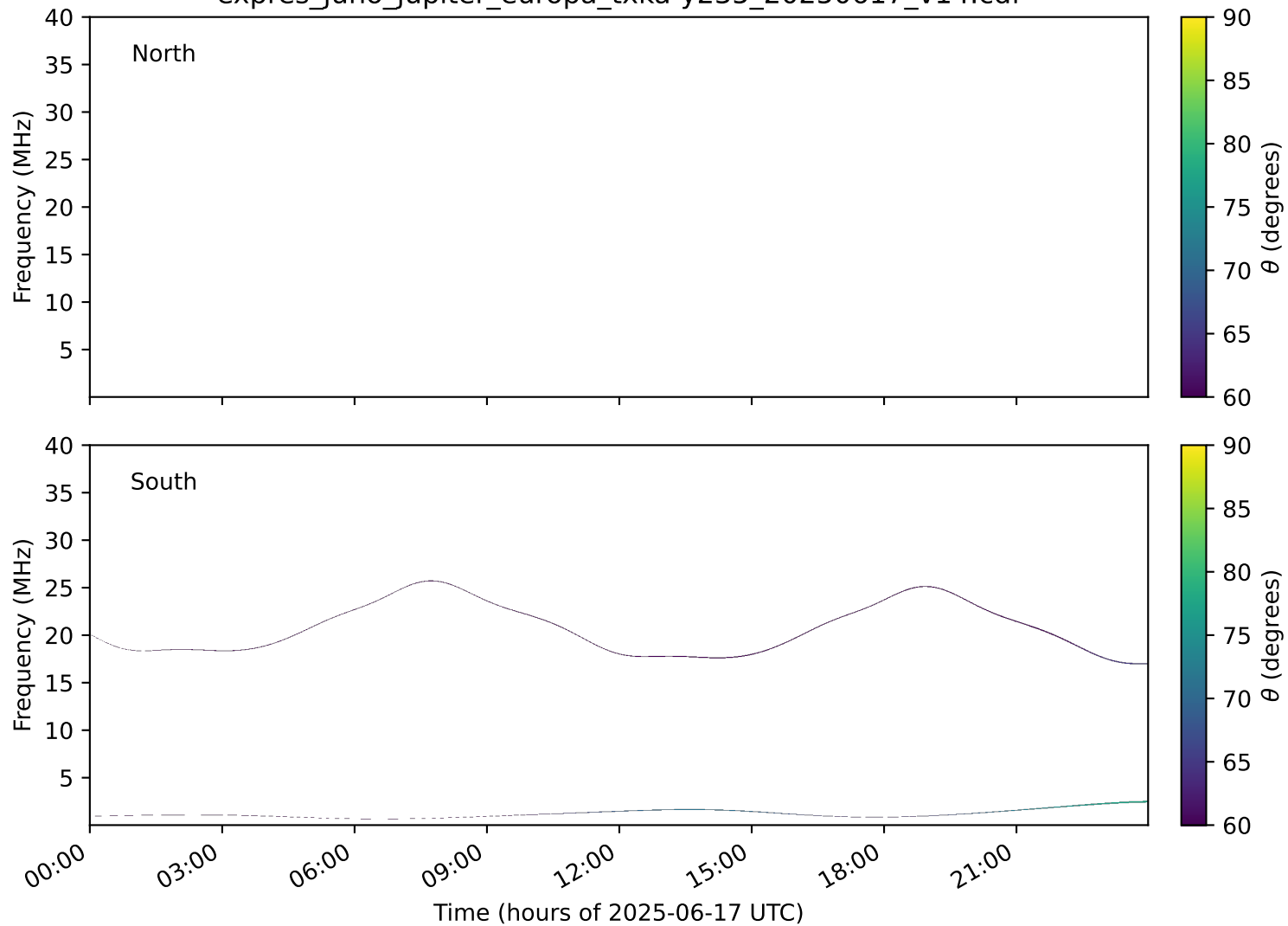
expres_juno_jupiter_europa_txka-y235_20250617_v14.cdf
