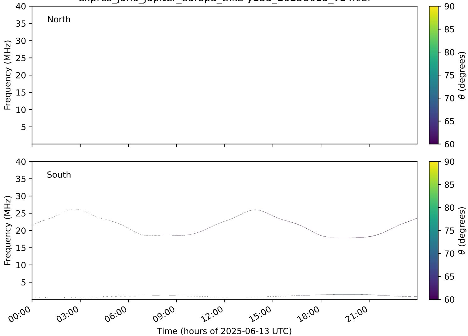
expres_juno_jupiter_europa_txka-y235_20250613_v14.cdf
