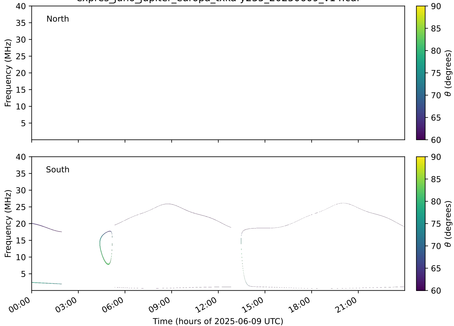
expres_juno_jupiter_europa_txka-y235_20250609_v14.cdf
