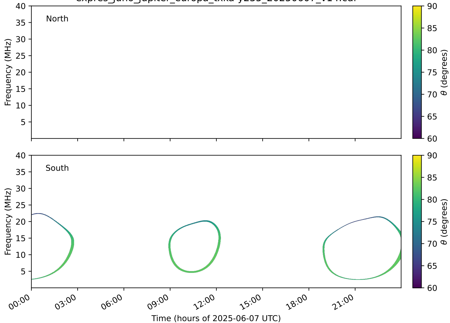
expres_juno_jupiter_europa_txka-y235_20250607_v14.cdf
