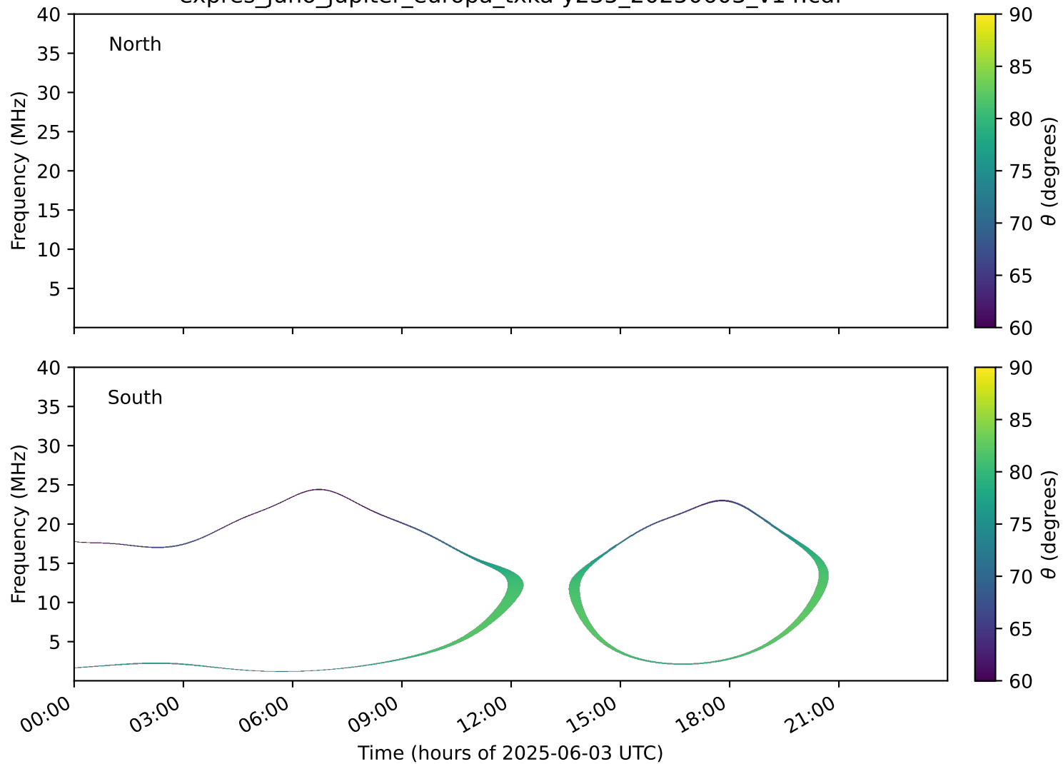
expres_juno_jupiter_europa_txka-y235_20250603_v14.cdf
