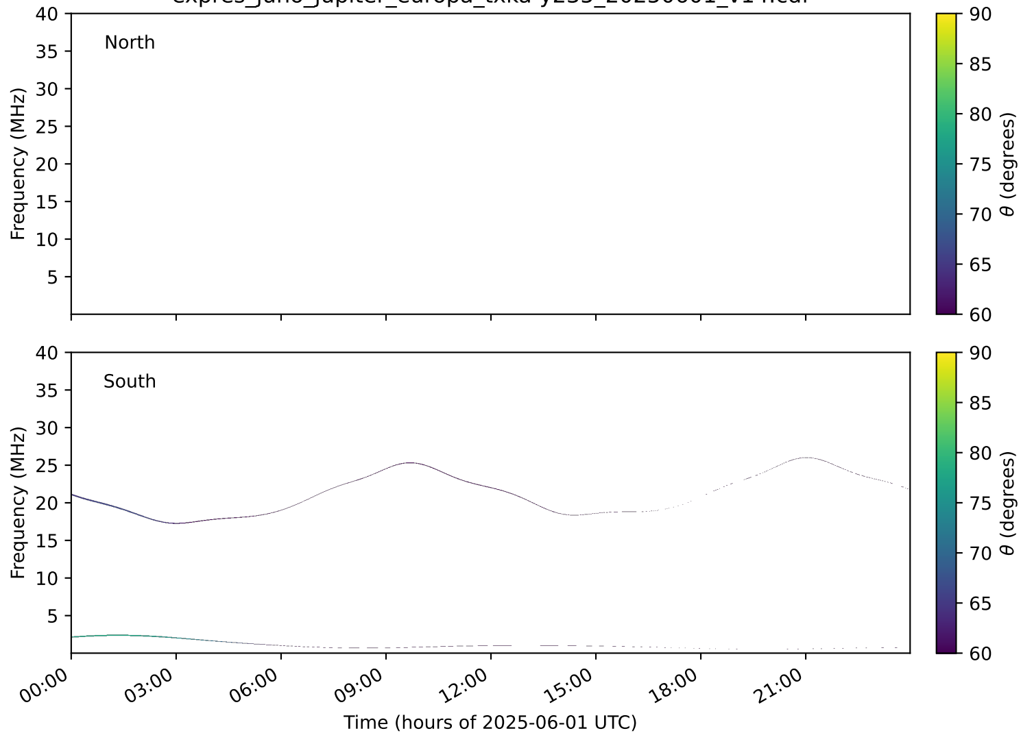
expres_juno_jupiter_europa_txka-y235_20250601_v14.cdf
