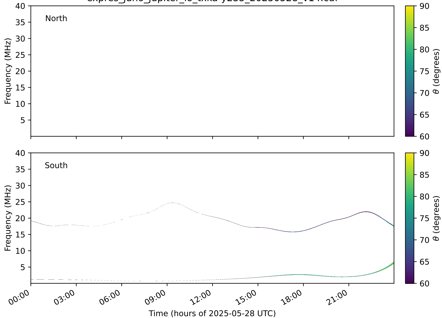
expres_juno_jupiter_io_txka-y235_20250528_v14.cdf
