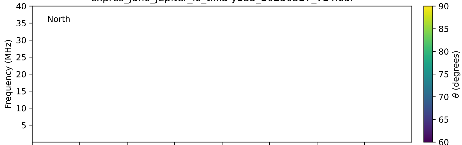
expres_juno_jupiter_io_txka-y235_20250527_v14.cdf
