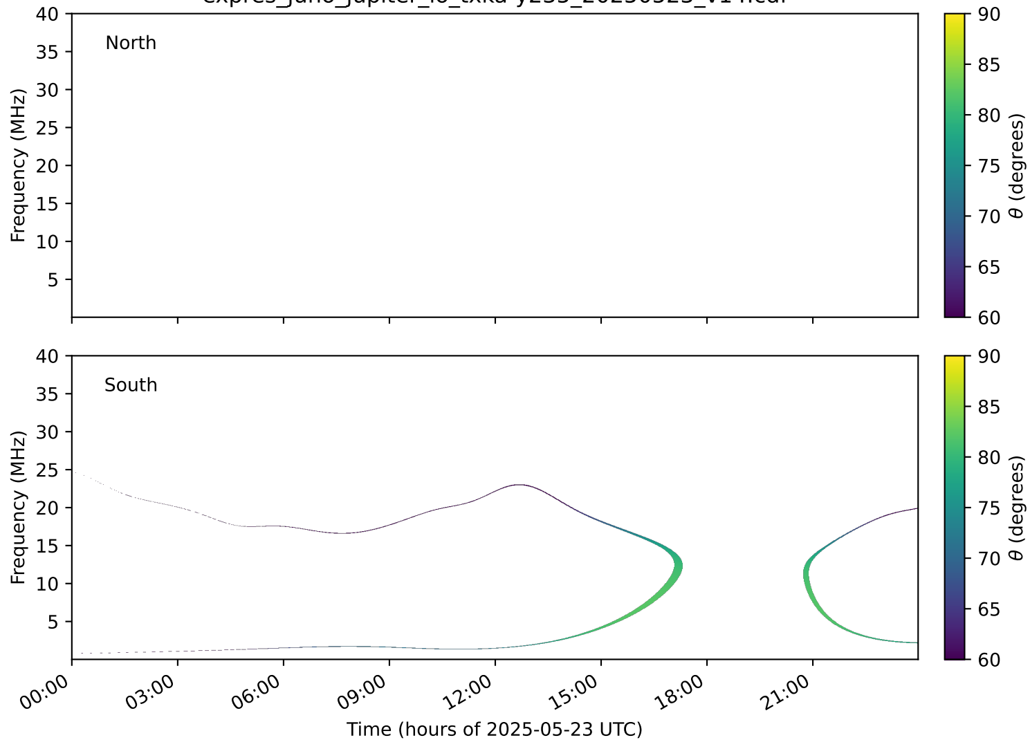
expres_juno_jupiter_io_txka-y235_20250523_v14.cdf
