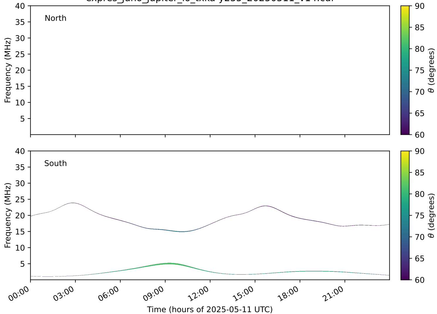
expres_juno_jupiter_io_txka-y235_20250511_v14.cdf
