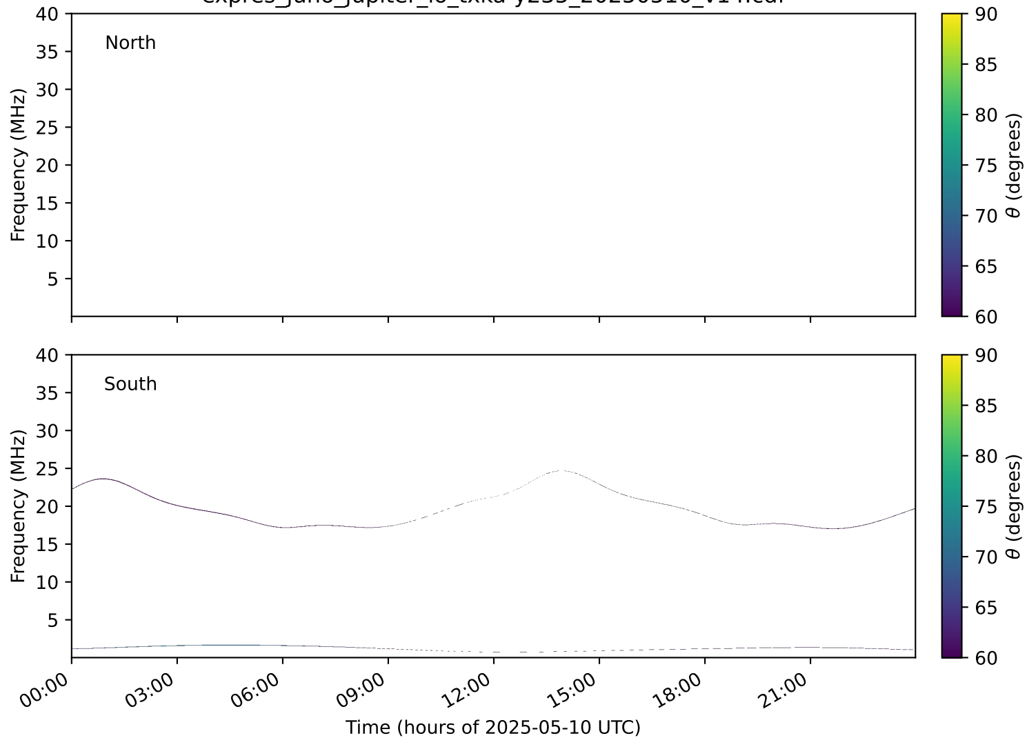
expres_juno_jupiter_io_txka-y235_20250510_v14.cdf
