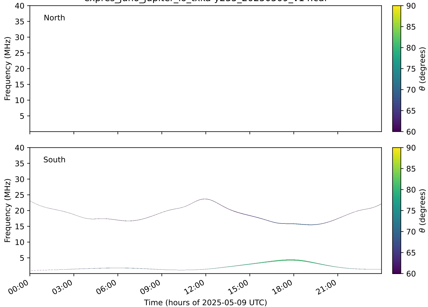
expres_juno_jupiter_io_txka-y235_20250509_v14.cdf
