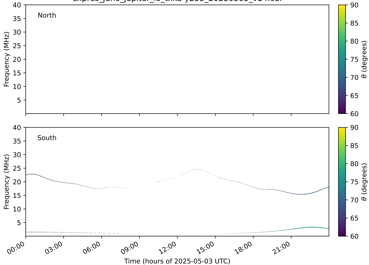
expres_juno_jupiter_io_txka-y235_20250503_v14.cdf
