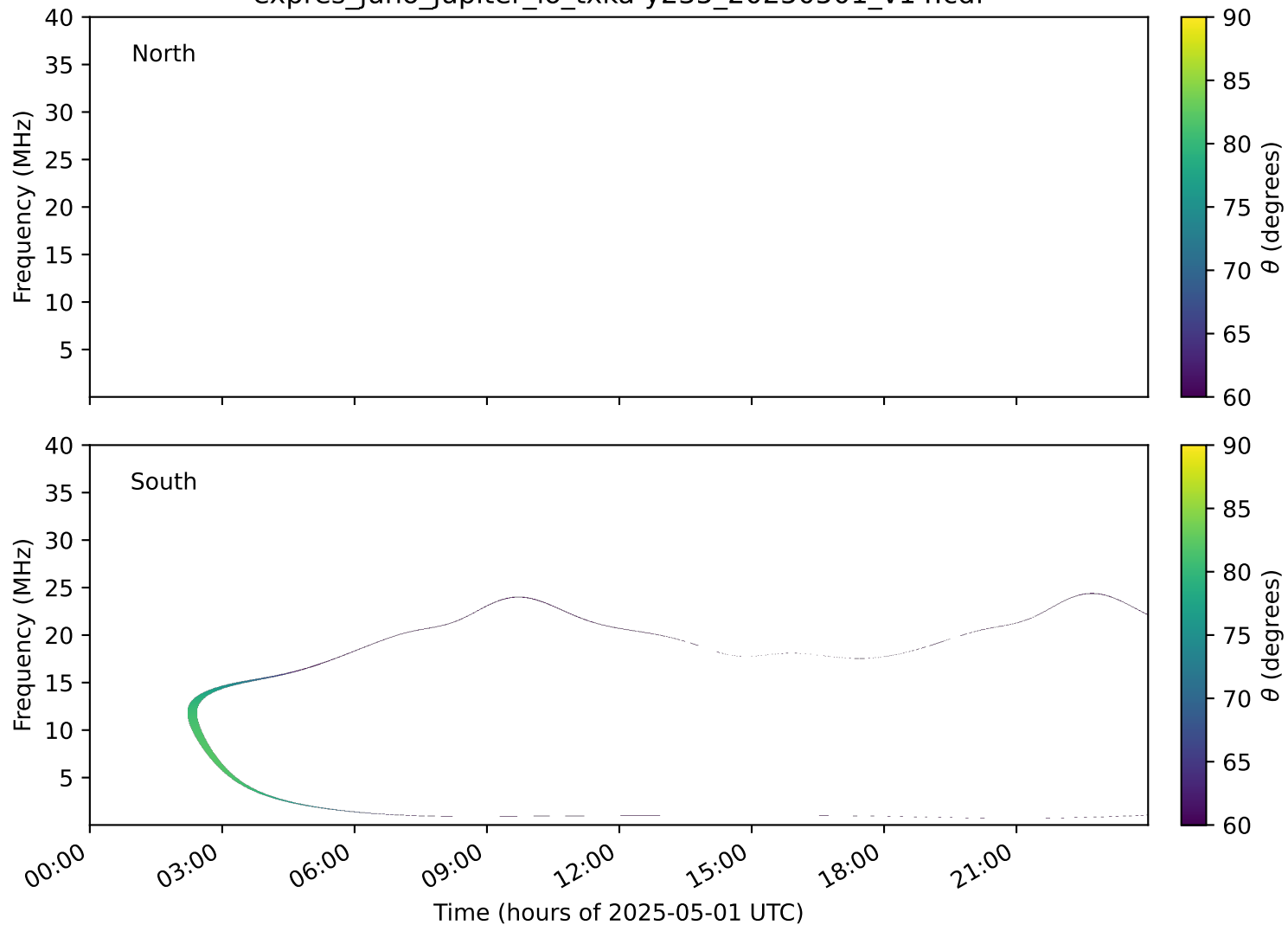
expres_juno_jupiter_io_txka-y235_20250501_v14.cdf
